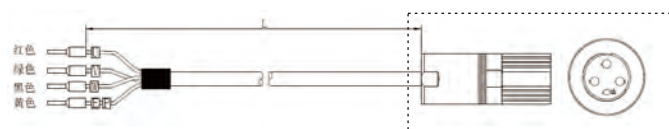
② CABLE-RZ*M*-HD(V2.0)绕组线
