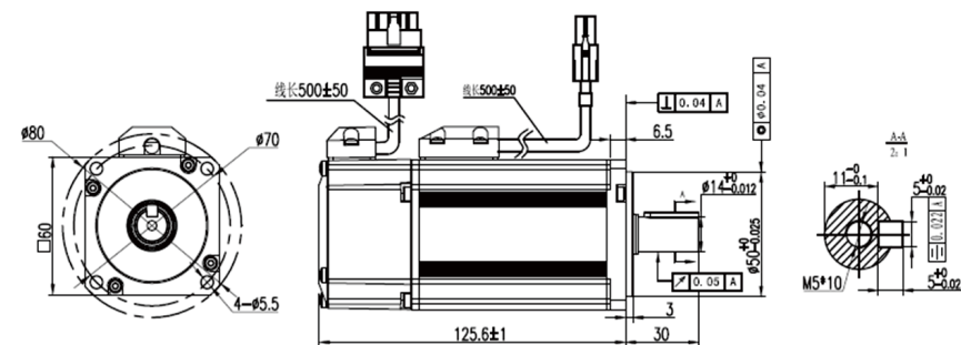
② 60机座电机安装尺寸400W
